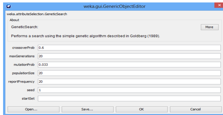
Figure 7: The Genetic Search Parameters
